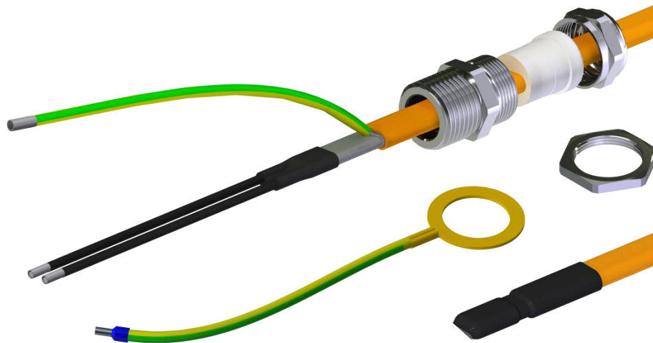
M20 cable gland kit with trace heater sealing and end seal for BARTEC PSB trace heaters
